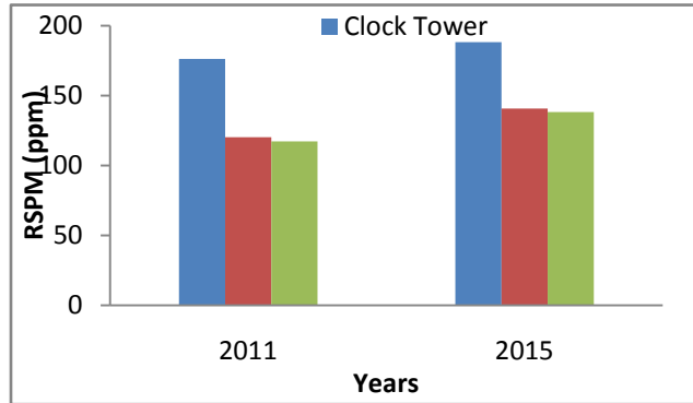
Fig. 5: Spatio-temporal Variation of RSPM during 2011 and 2015
